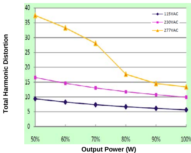
Figure 9: Total Harmonic Distortion vs. Output Power
